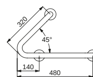
Left model - 5181G
