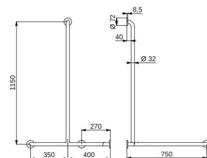
Left model - 5481G
