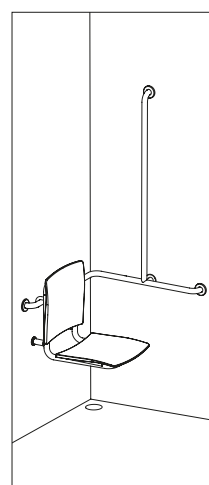
Installation example for showers
