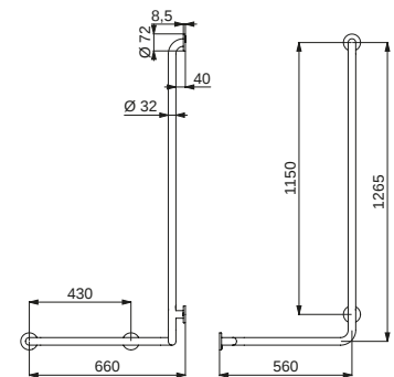
Left model - 5100G
