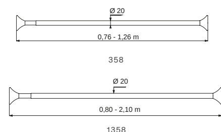
Telescopic, straight curtain rail
