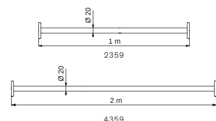
Straight curtain rail, cut-to-size - Concealed fixings
