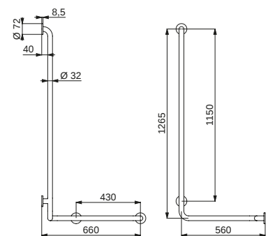
Right model - 5100D
