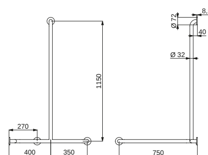
Right model - 5481D
