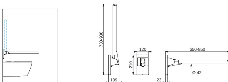
Installation example for WCs
