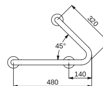
Right model - 5181D
