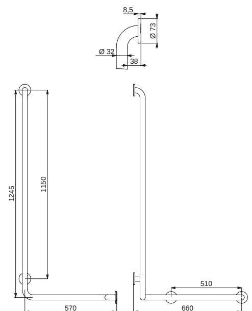
Installation example for showers
