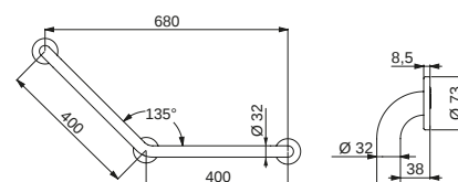
Installation example for WCs
